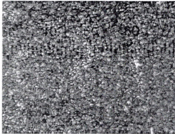
Figure 2: spheroidal carbide + martensite (small punch**)
