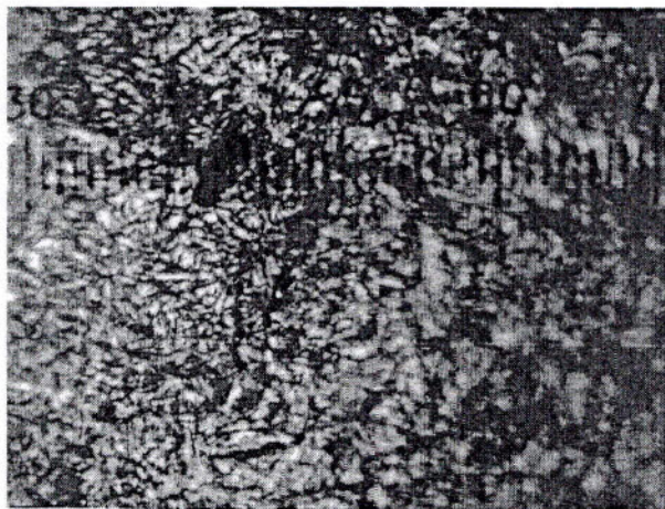
Figure 3: retain austenite + martensite (large punch)
