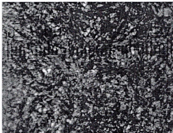
Figure 1: retain austenite + martensite (small punch*)
